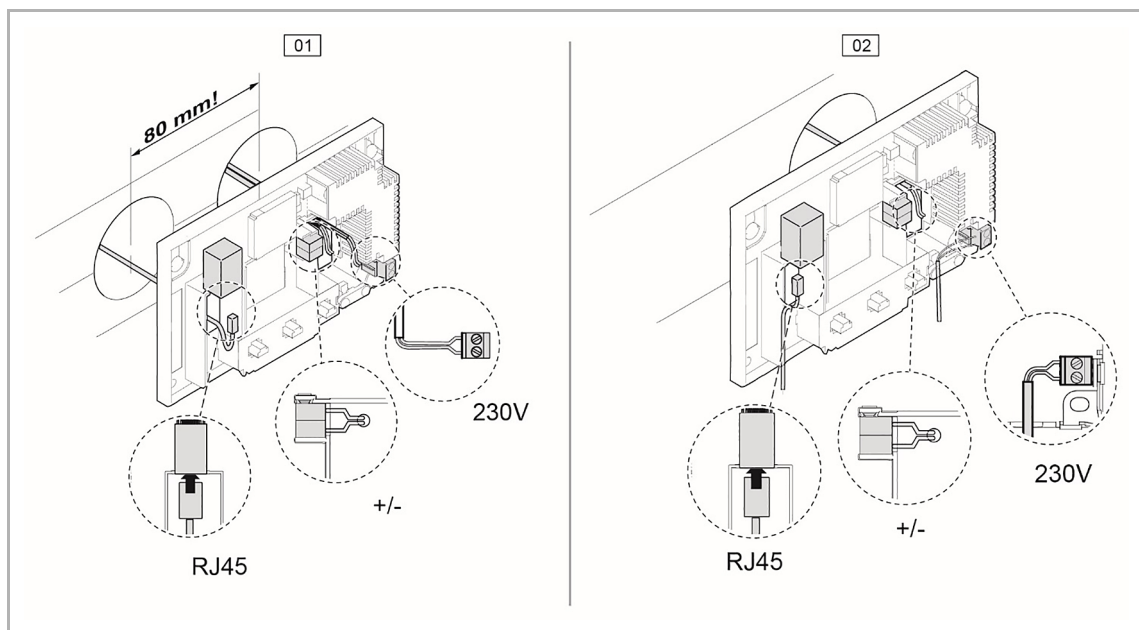
Fig. 91: Mounting the System Access Point
