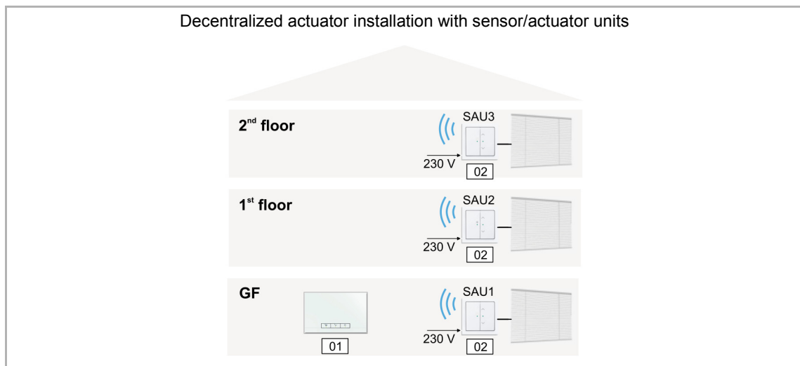
Fig. 6: Planning of the wireless actuators
