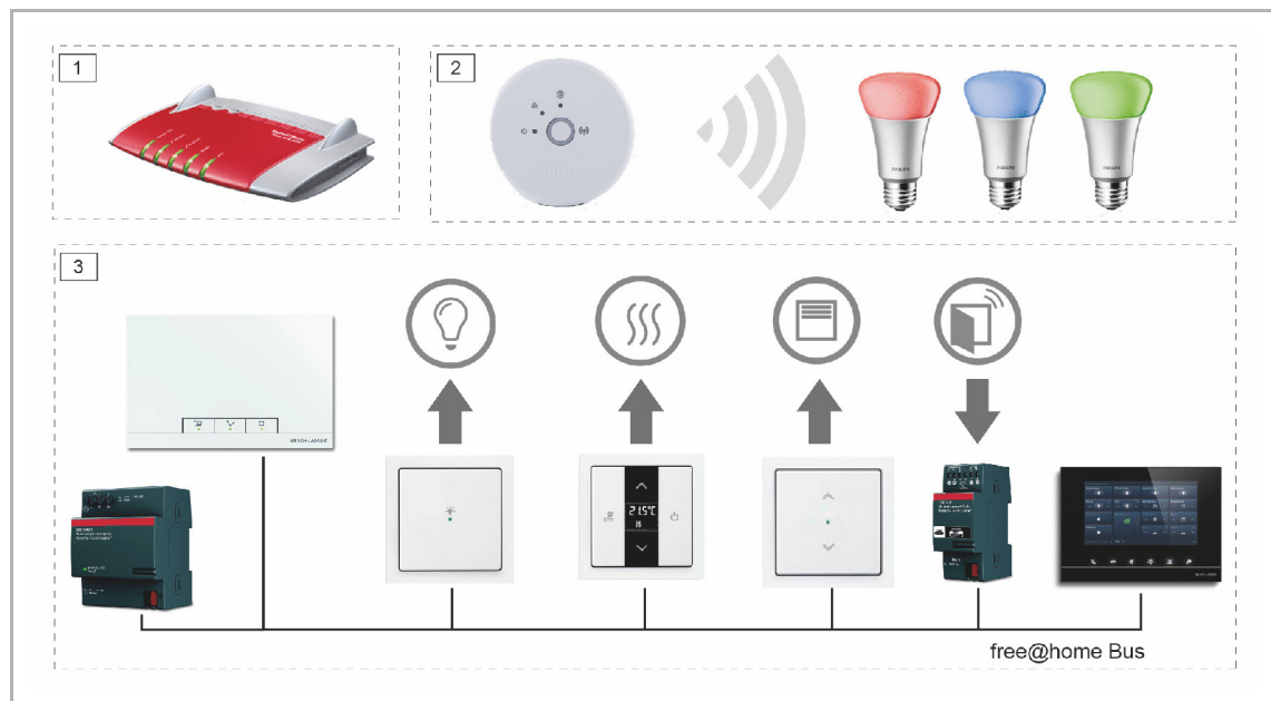
Fig. 80: Philips Hue Integration
