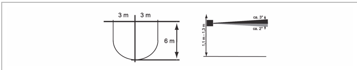
Fig. 62: Detection range
