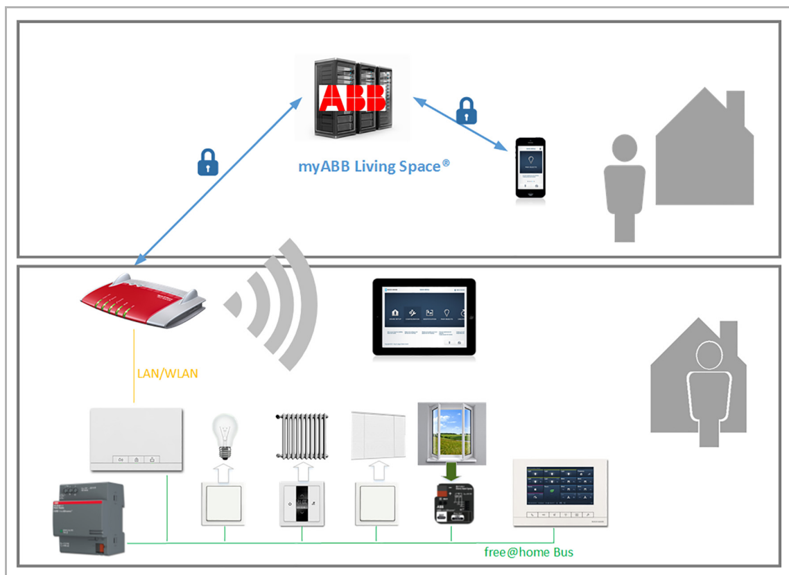
Fig. 39: myABB Living Space® Topology
